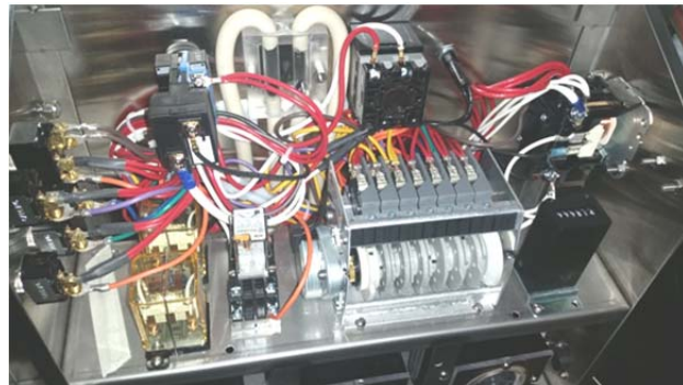
ASQ control box with cover removed
