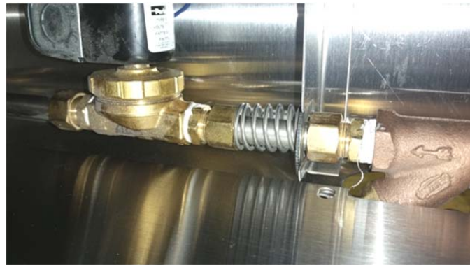
Showing 1/2" H2O solenoid, also stainless 1.5" drain tube
